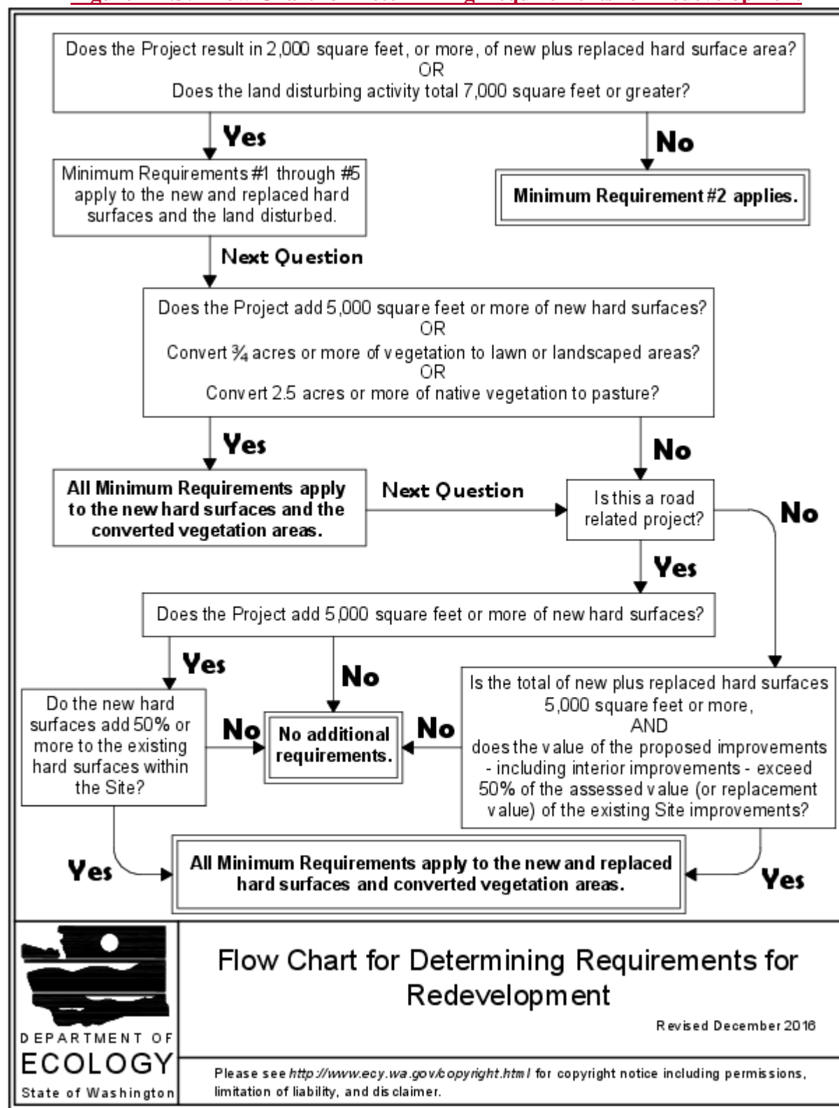
Figure 1-4.3: Flow Chart for Determining Requirements for Redevelopment
